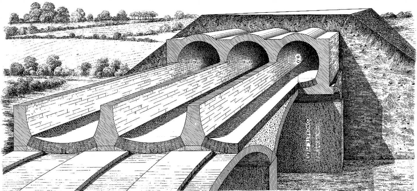
NORTHERN OUTFALL SEWER. SECTION OF EMBANKMENT, CULVERTS AND SUBSTRUCTURE.
