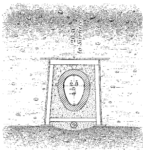
SECTION OF SEWER IN TUNNEL NEAR THE UPPER MALL, HAMMERSMITH.
