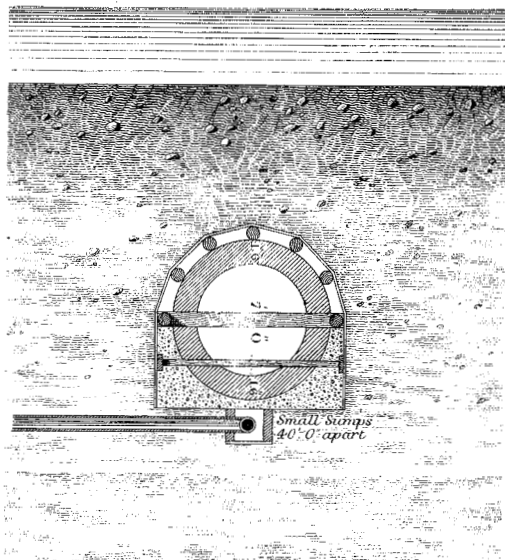
SECTION OF SEWER IN TUNNEL UNDER GRAND SURREY CANAL.
