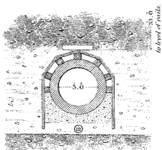
SECTION OF SEWER IN TUNNEL UNDER WEST LONDON RAILWAY, NEAR FULHAM GAS WORKS.
