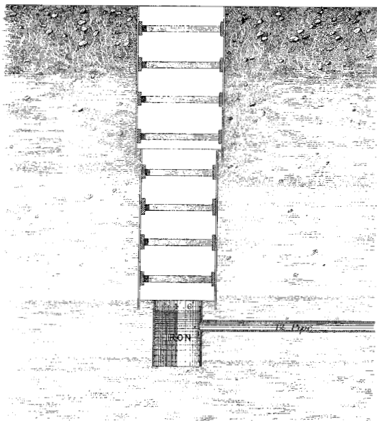
SECTION OF SUMP, OLD KENT ROAD, NEAR GRAND SURREY CANAL.
