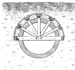
SECTION OF SEWER IN TUNNEL UNDER NEW RIVER EMBANKMENT.
