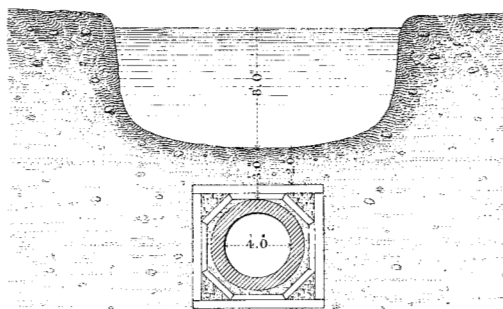
SECTION OF SEWER IN TUNNEL UNDER REGENT'S CANAL, CALEDONIAN ROAD.
