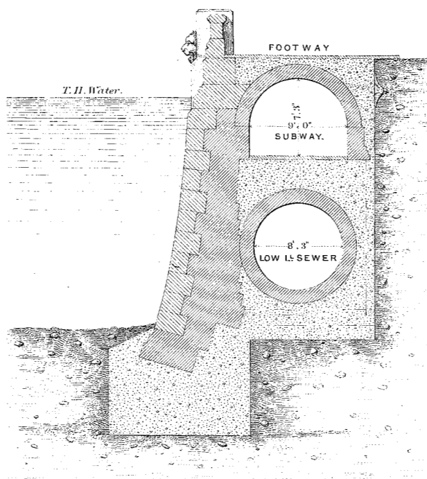
SECTION OF THAMES EMBANKMENT, SUBWAY & LOW LEVEL SEWER.
