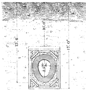
SECTION OF SEWER IN TUNNEL UNDER HORSE GUARDS.
