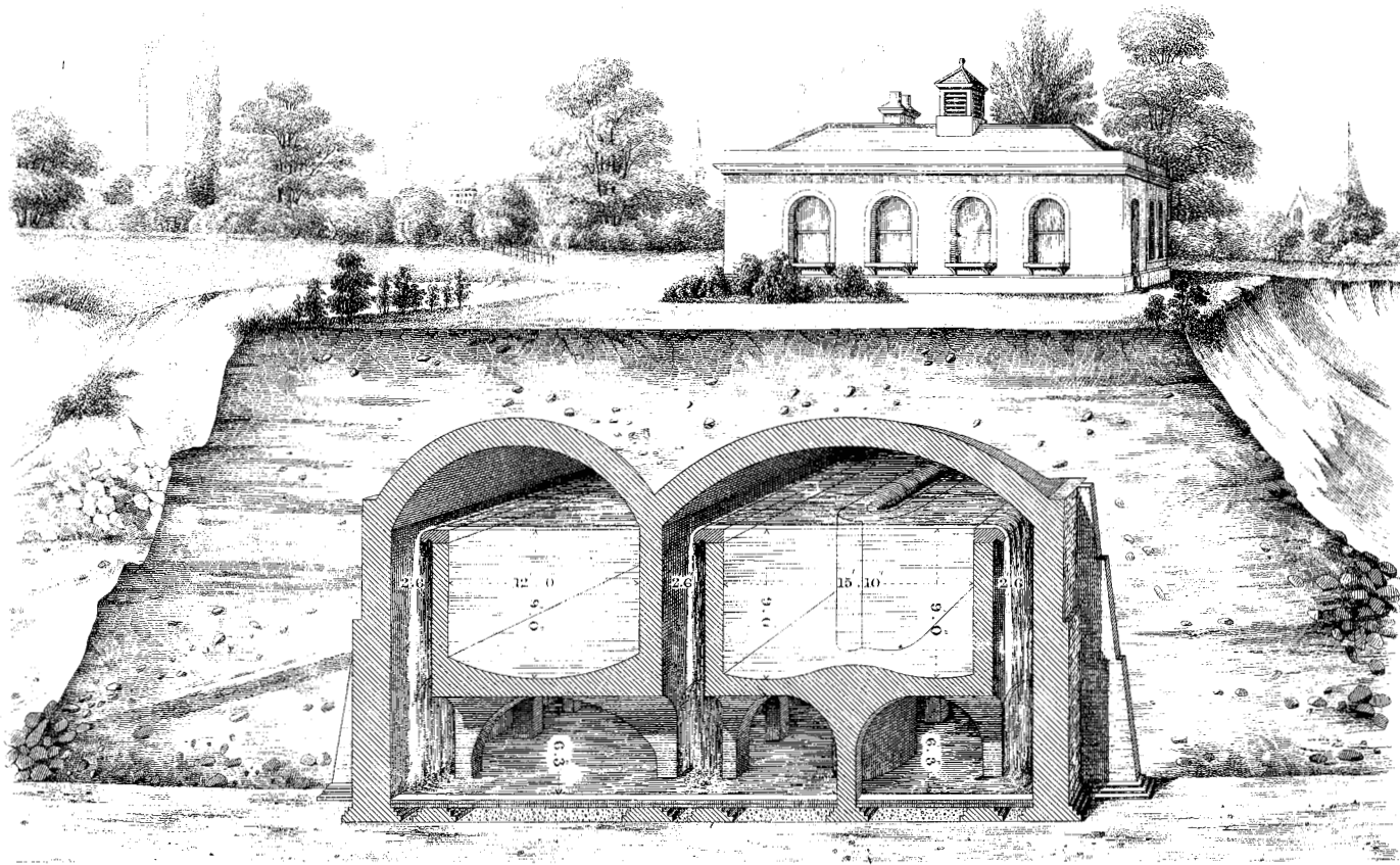
SECTION OF OVERFLOW CHAMBER AT JUNCTION OF NORTHERN HIGH & MIDDLE LEVEL SEWERS.
