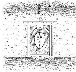
SECTION OF SEWER IN TUNNEL UNDER QUEEN STREET, HAMMERSMITH.
