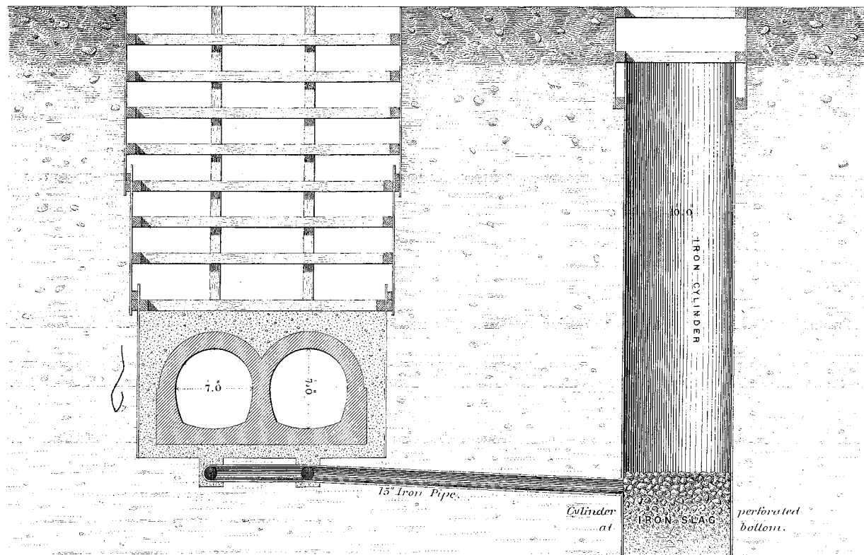
LOW LEVEL SEWER AT GAS WORKS, DEPTFORD. TRANSVERSE SECTION OF SEWER & SUMP.
